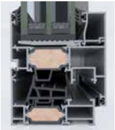
Level 2 Uf: ≥1.2 W/m²K
