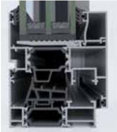
Level 1 Uf: ≥1.8 W/m²K
