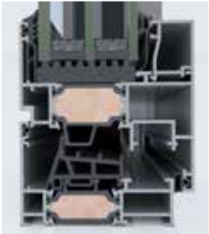
Level 3 Uf: ≥1.1 W/m²K
